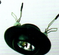
EB 619 BLACK DIAM 3.54" HEIGHT 2.48" MR16
